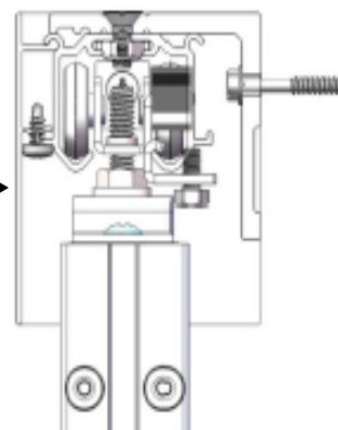
SIDE VIEW TOP ROLLER
