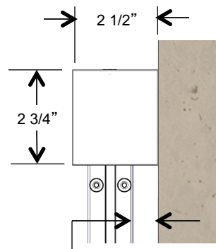
SIDE VIEW BOTTOM ROLLER
